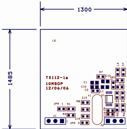
Assembly Drawing MICRF112 Demo Board
