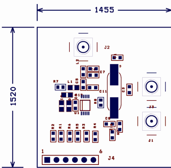
Assembly Drawing MICRF112 50 Ohm Test Board
