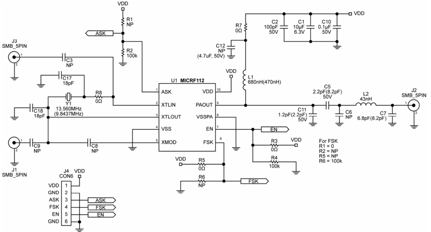
Figure 2. MICRF112 Test Circuit with 50Ω Output
