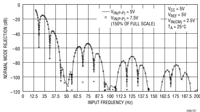
Figure 26. Measure Input Normal Mode Rejection vs Input Frequency with Input Perturbation of 150% (50Hz Notch)
