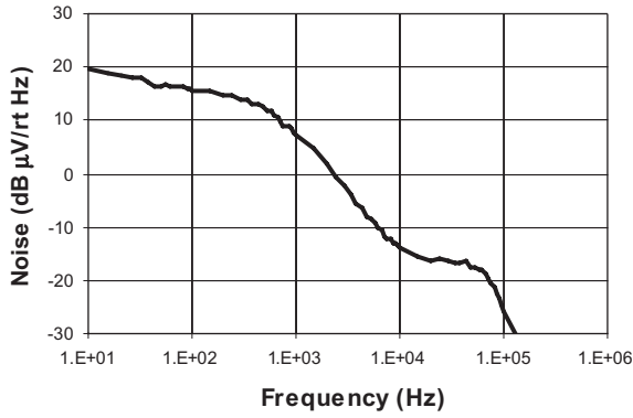
Noise Spectrum
