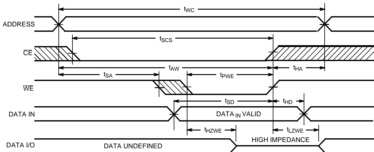
Write Cycle No.1 ( \overline{WE} Controlled) [8]
