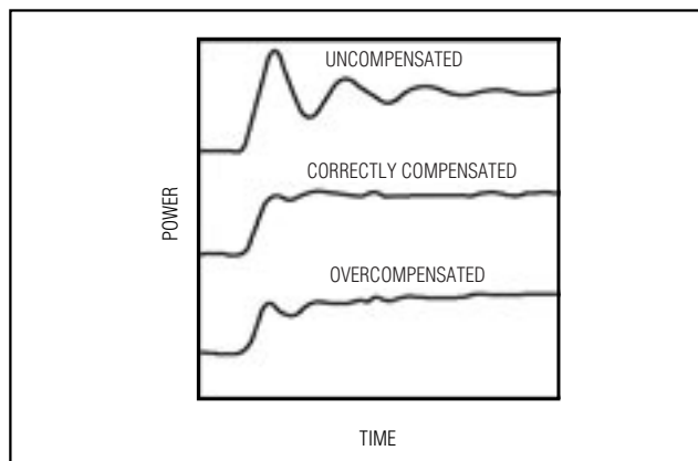
Figure 7. Laser Compensation
