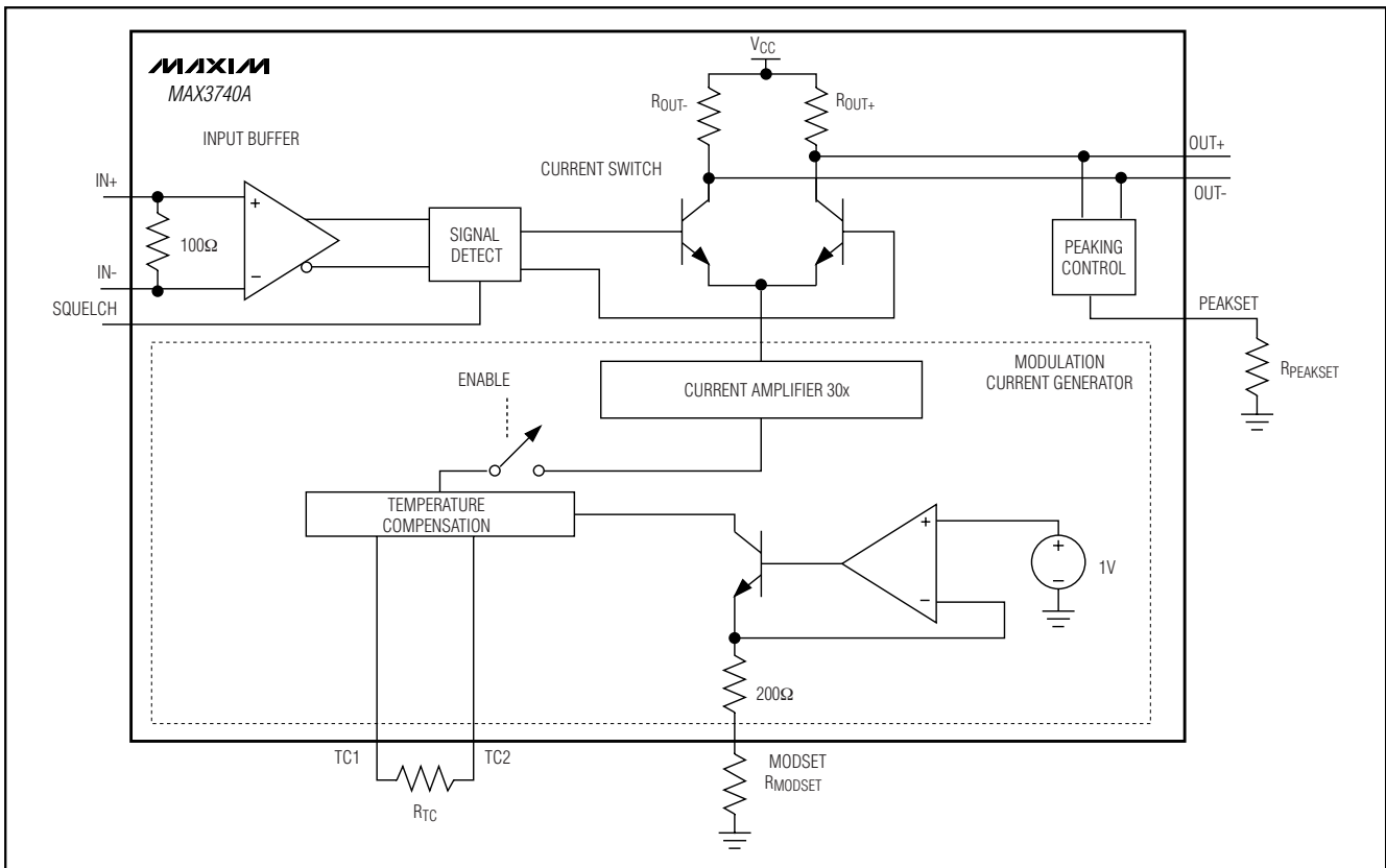
Figure 3. Modulation Circuit
