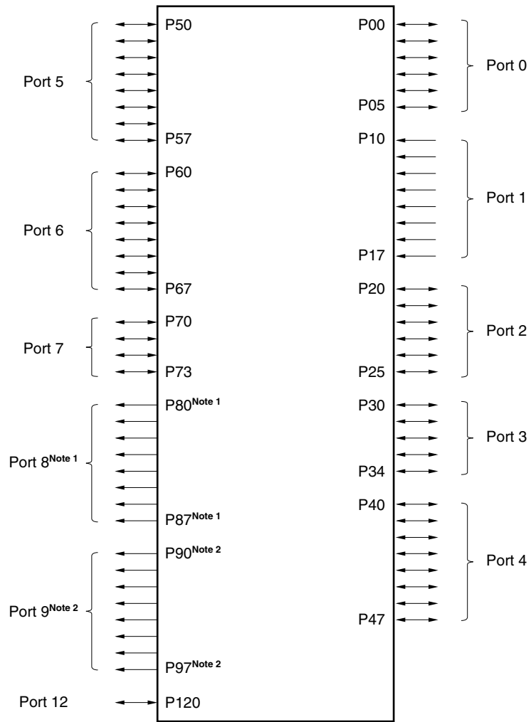
Figure 4-1. Port Types
