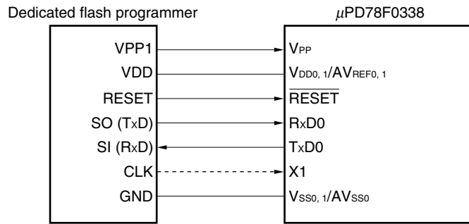
Figure 22-6. UART (UART0)
