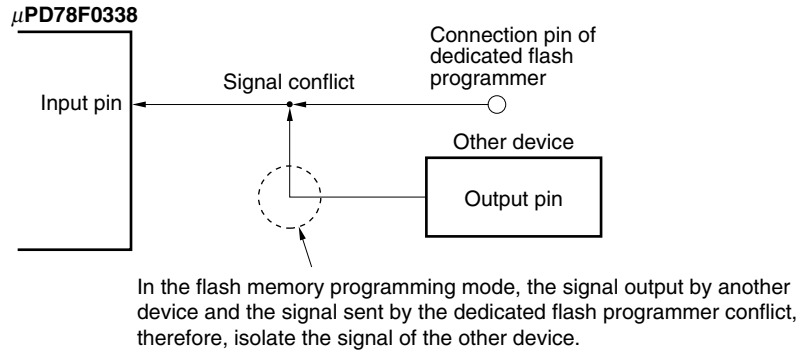
Figure 22-8. Signal Conflict (Input Pin of Serial Interface)
