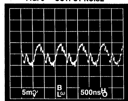
FIG. 3 — OUTPUT NOISE
