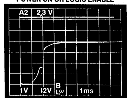
FIG. 6 — TURN-ON TIME POWER ON OR LOGIC ENABLE
