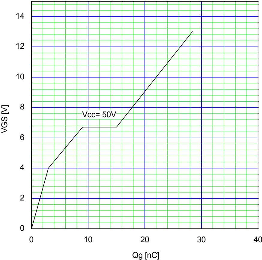
Typical Gate Charge Characteristics V_{GS}=f(Q_g):I_D=20A,T_{ch}=25^{\circ}C
