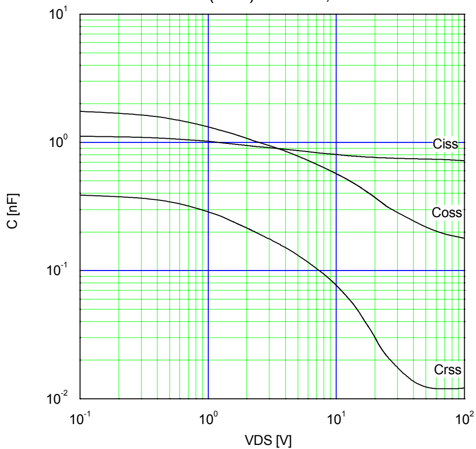
Typical Capacitance C=f(V_{DS}):V_{GS}=0V, f=1MHz
