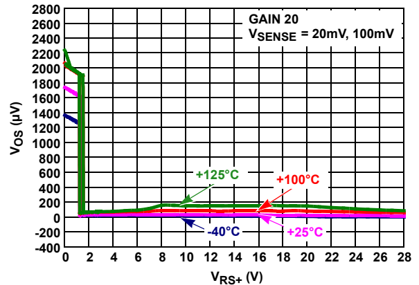
FIGURE 34. V_{OS} vs V_{RS+}
