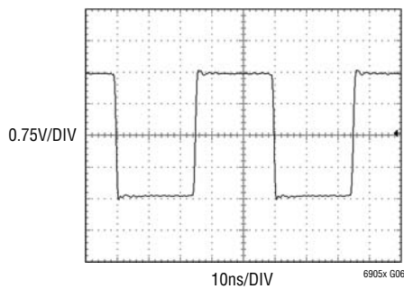
LTC6905-80 Output Operating at 20MHz, V_S = 3V
