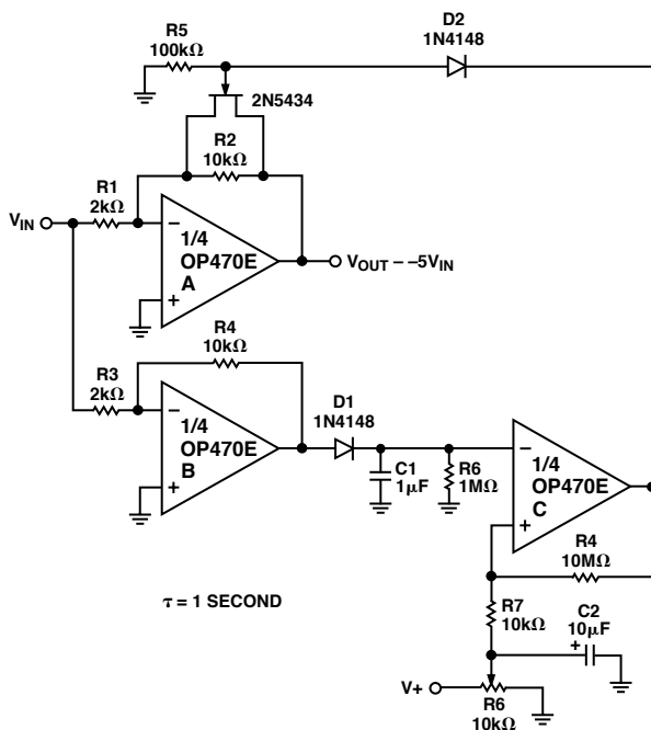
Figure 17. Squelch Amplifier
