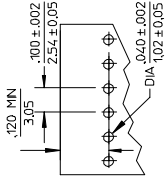
RECOMMENDED PC BOARD LAYOUT
