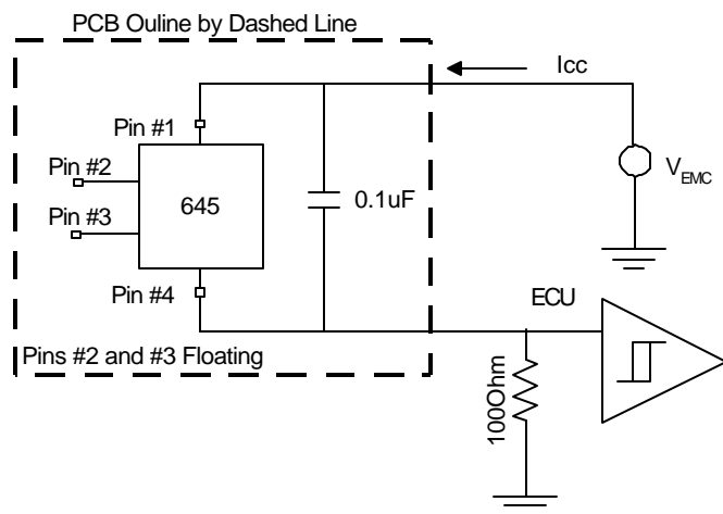
Transient & EMC test circuit
