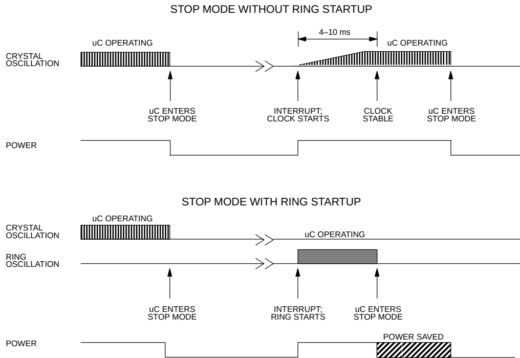
RING OSCILLATOR START-UP Figure 4
