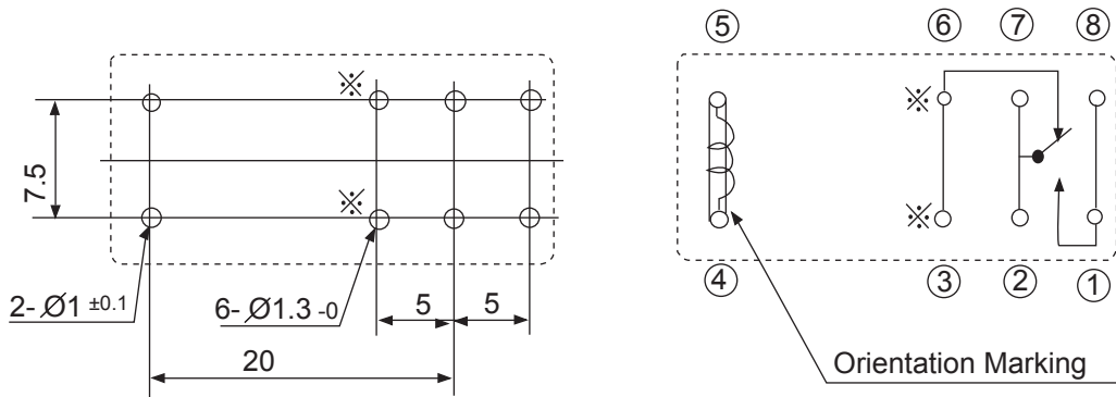
I PC Board mounting hole layout (BOTTOM VIEW)
