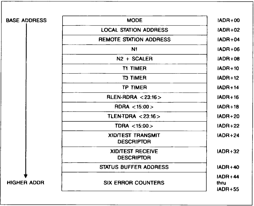
Figure 6 : Initialization Block.
