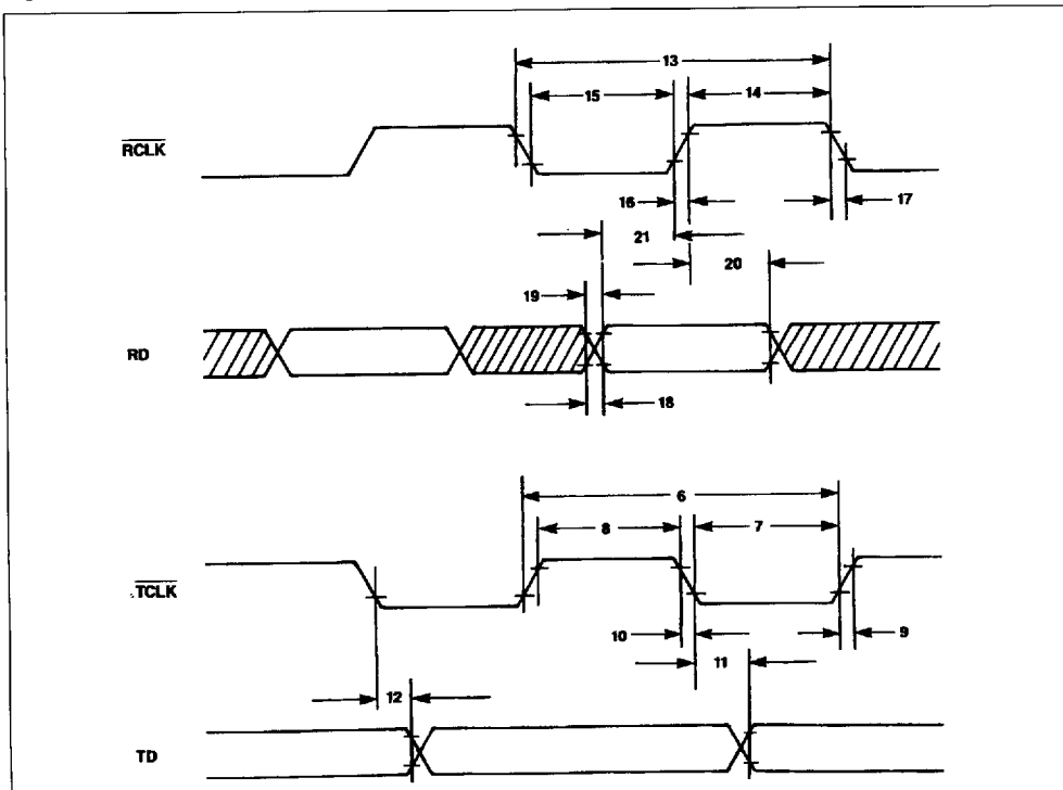
Figure 9 : Serial Link Timing Diagram.
