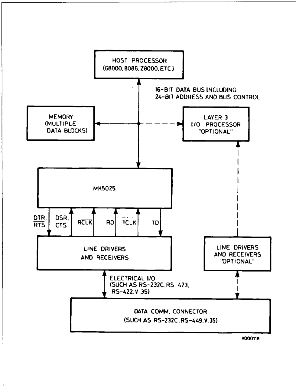
Figure 3 : Possible System Configuration for the MK5025.
