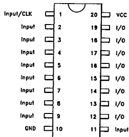
Pin Names
