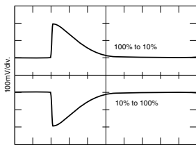
SMHF2805S STEP LOAD RESPONSE
