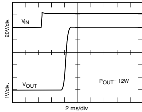
SMHF2805S TURN-ON INTO FULL LOAD
