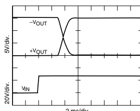
SMHF2815D TURN-ON INTO FULL LOAD
