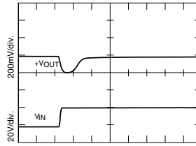
SMHF2815D STEP LINE RESPONSE
