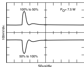
SMHF2815D STEP LOAD RESPONSE
