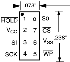
8-Lead XBGA: Top View
