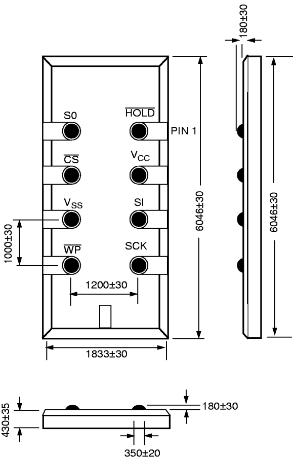
X25138: Bottom View
