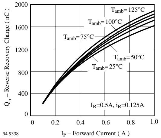
Figure 7. Typ. Reverse Recovery Charge vs. Forward Current
