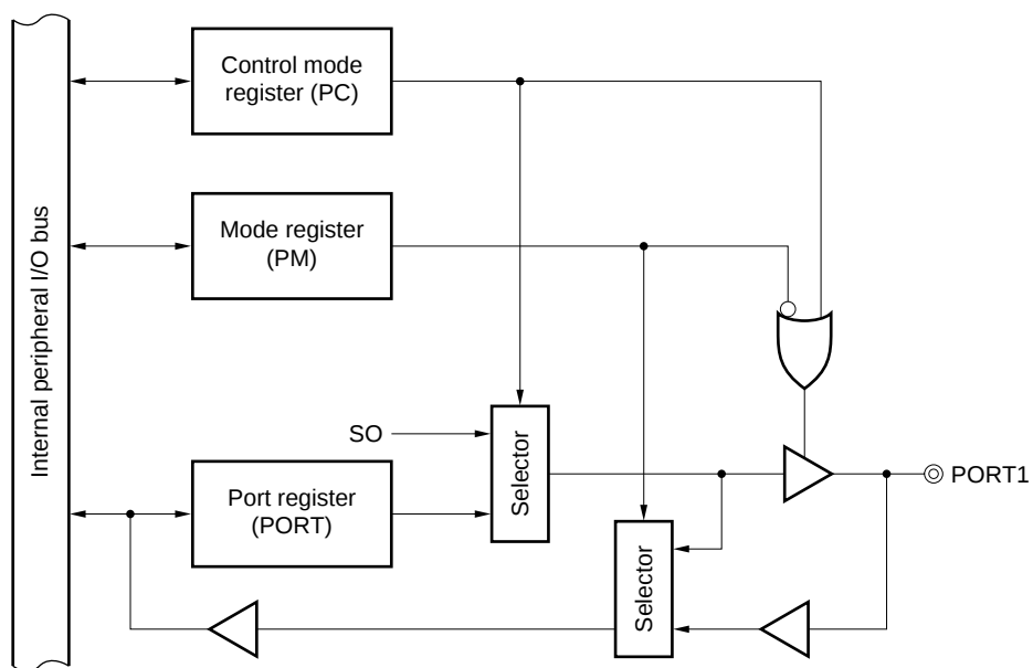
Figure 11-2. Block Diagram of Port 1
