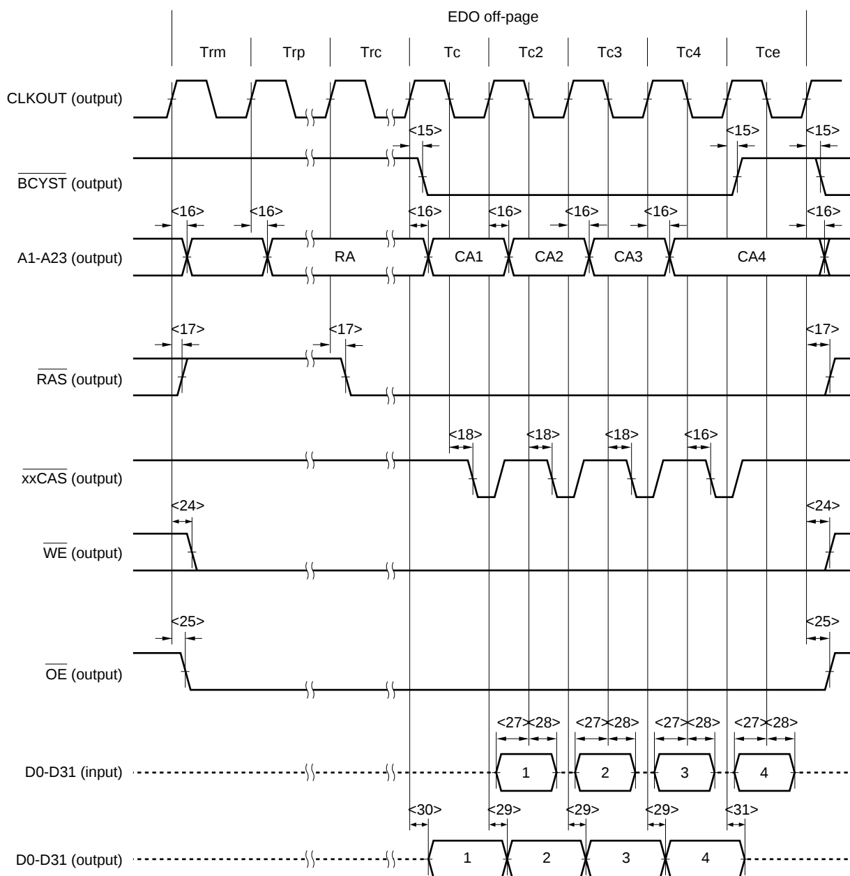
(g) DRAM burst 1-clock \overline{\text{CAS}} off-page cycle (32-bit data bus)
