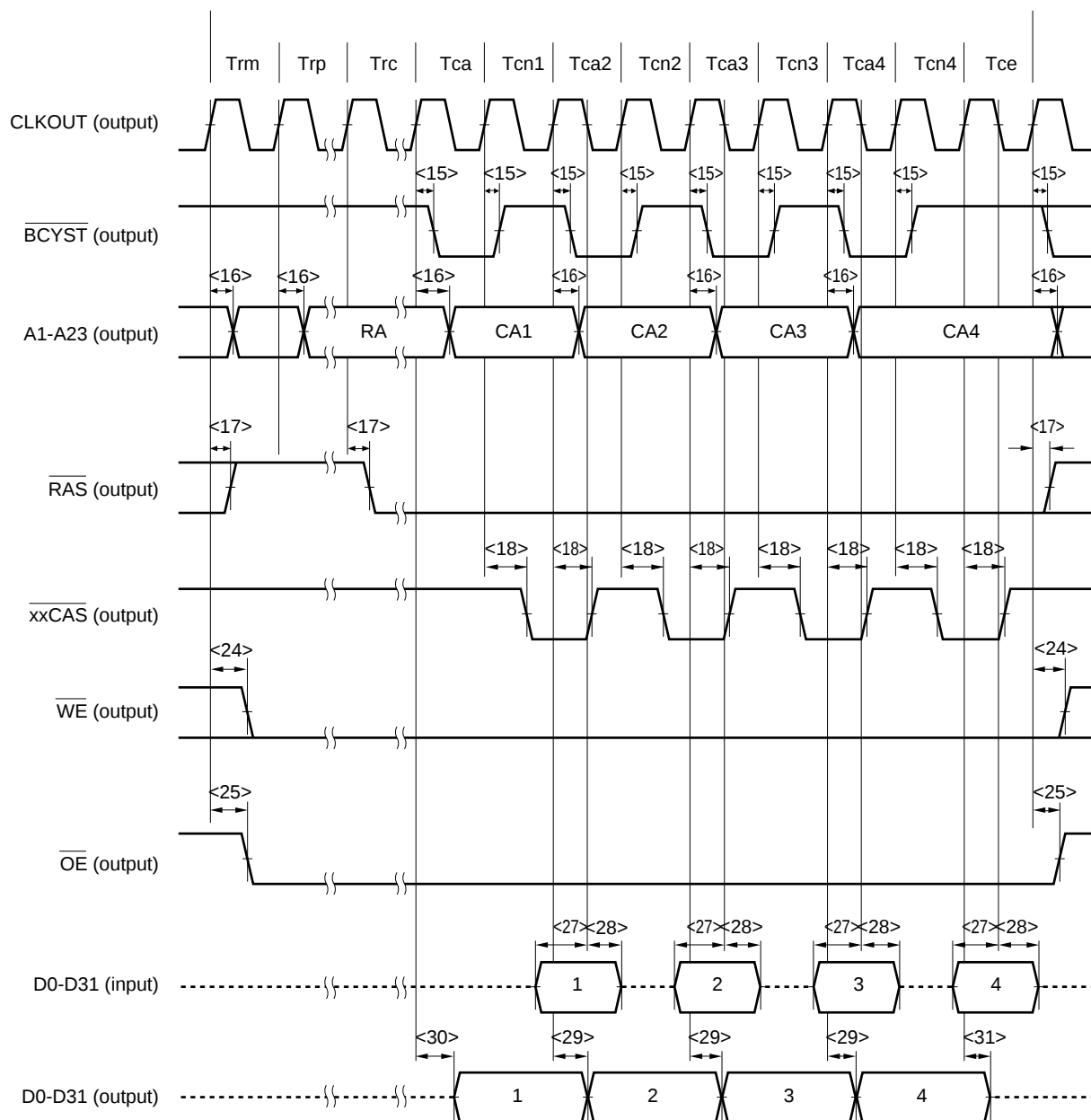
(h) DRAM burst 2-clock \overline{\text{CAS}} off-page cycle (32-bit data bus)
