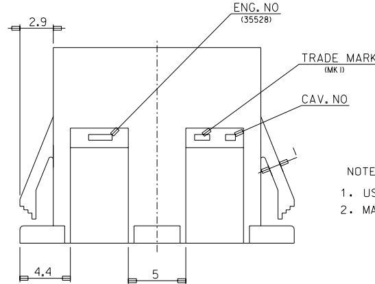
SECTION E-E
