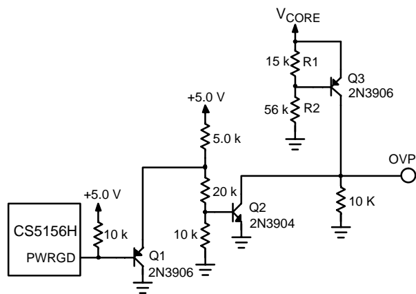
Figure 22. Circuit To Implement A Dedicated OVP Output Using The CS516H
