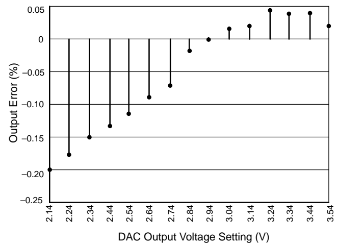
Figure 8. Percent Output Error vs. DAC Output Voltage Setting V_{CC} = 12\text{ V} , T_A = 25^\circ\text{C} , V_{ID4} = 1
