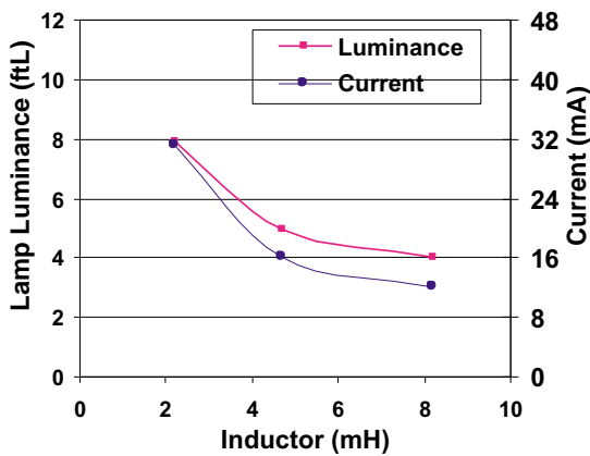
Figure 5: V+=5.0V, 4 in 2 EL Lamp
