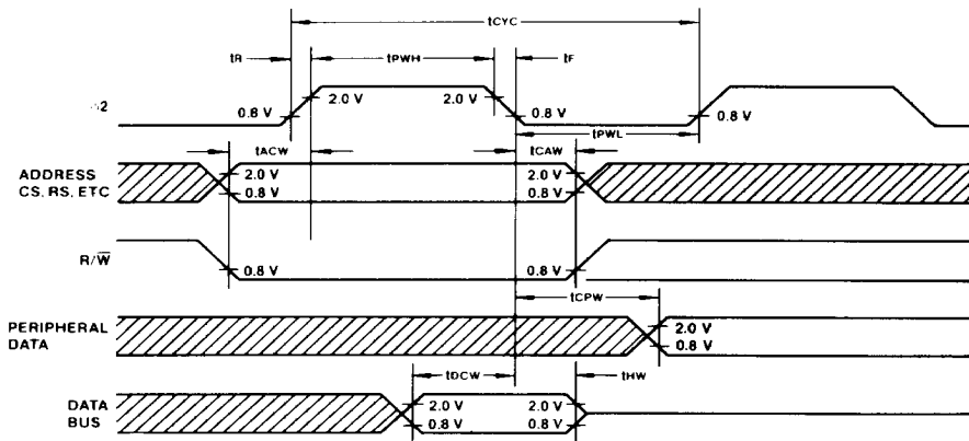
Figure 2. Write Timing
