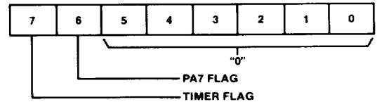
Figure 5. Interrupt Flag Register
