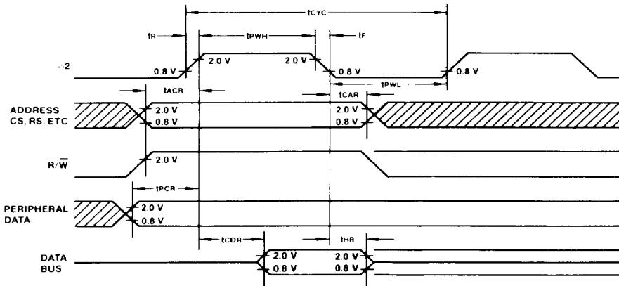
Figure 1. Read Timing
