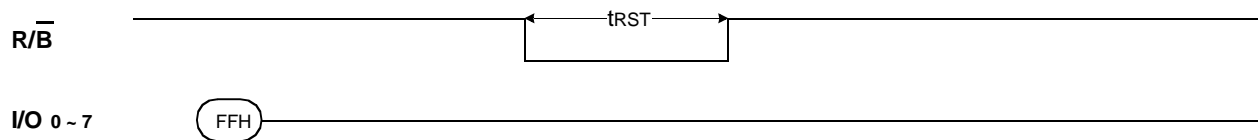
Figure 10. RESET Operation
