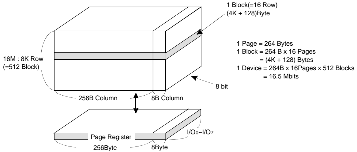
Figure 2. ARRAY ORGANIZATION
