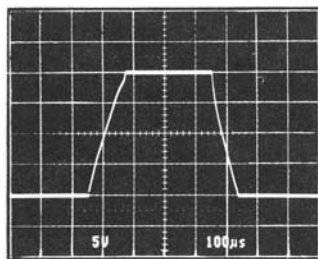
\begin{aligned} T_A &= 25^\circ\text{C} \\ V_S &= \pm 15\text{V} \\ A_V &= +1 \end{aligned}
