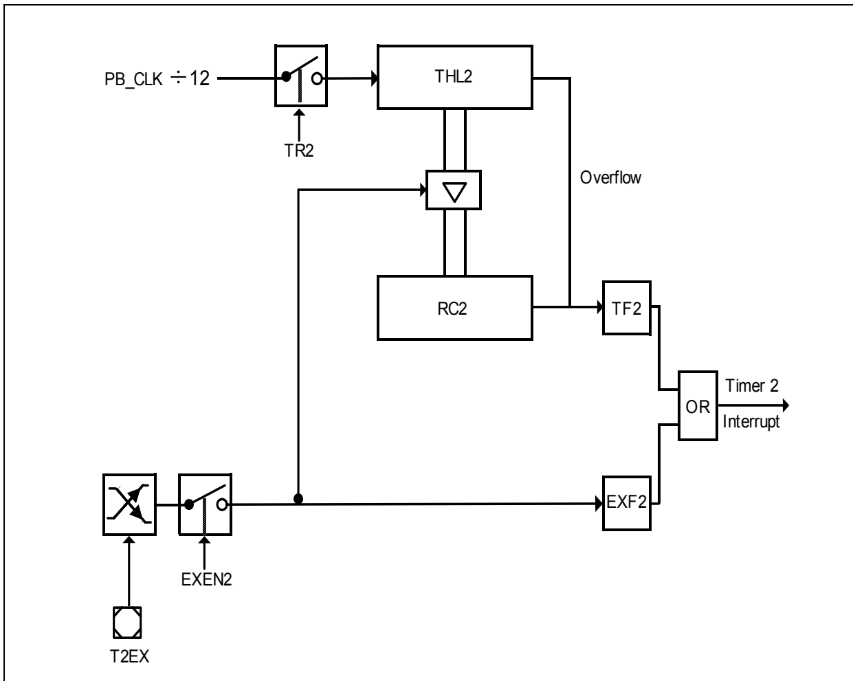
Figure 11-7 Capture Mode
