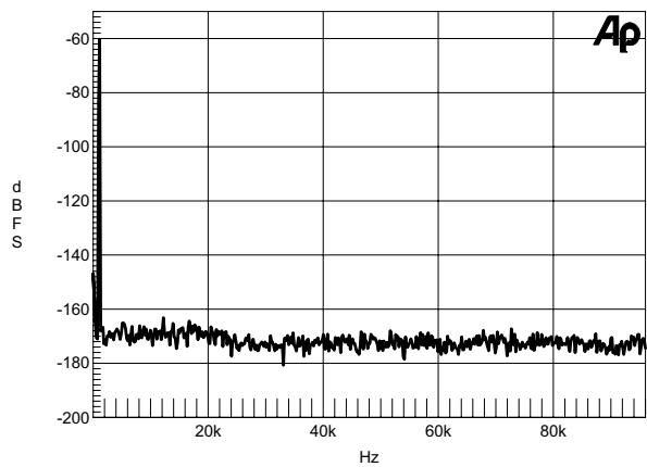
Figure 19b. Wideband FFT Plot (16k Points) -60 dBFS 1 kHz Tone, 44.1 kHz:192 kHz
