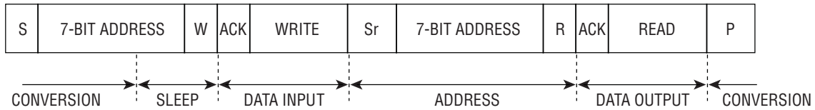
Figure 8. Write, Read, Start Conversion
