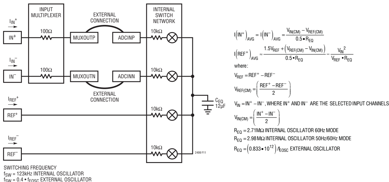
Figure 11. Equivalent Analog Input Circuit
