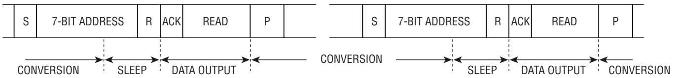
Figure 7. Consecutive Reading with the Same Input/Configuration
