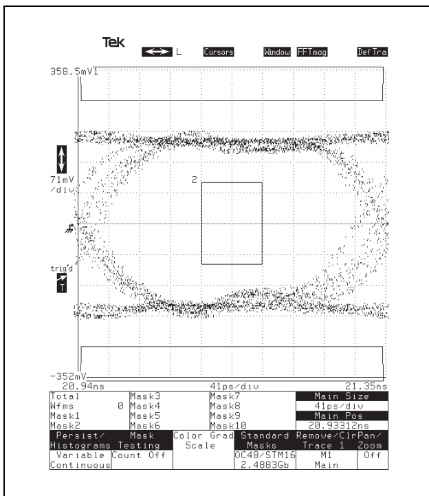
Figure 4 P_{opt} = 100 \mu\text{W avg.} (OC-48/STM-16)
