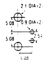
RIGHT ANGLE MOUNTING
