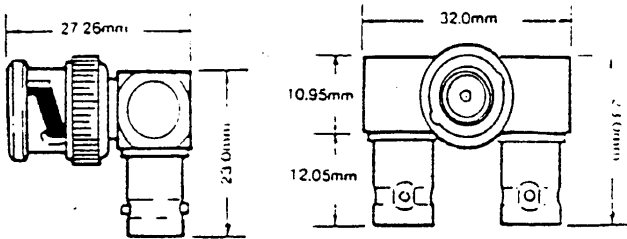
ORDER NO 251070 RIGHT ANGLE PLUG TO (2) JACKS
