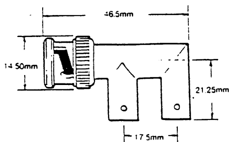
ORDER NO 251197 BNC PLUG TO (2) JACKS
