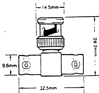
ORDER NO 251197 BNC PLUG TO (2) JACKS
