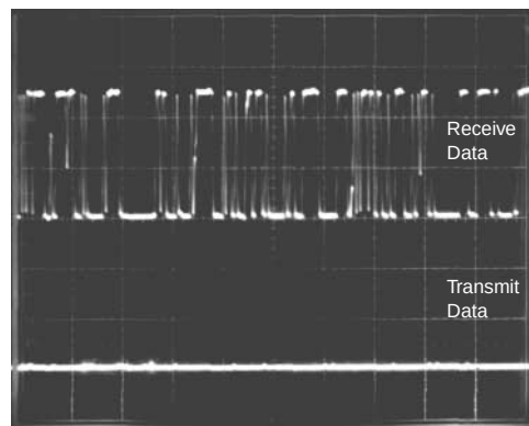
Figure 6. Receive Noise with No RF Signal
