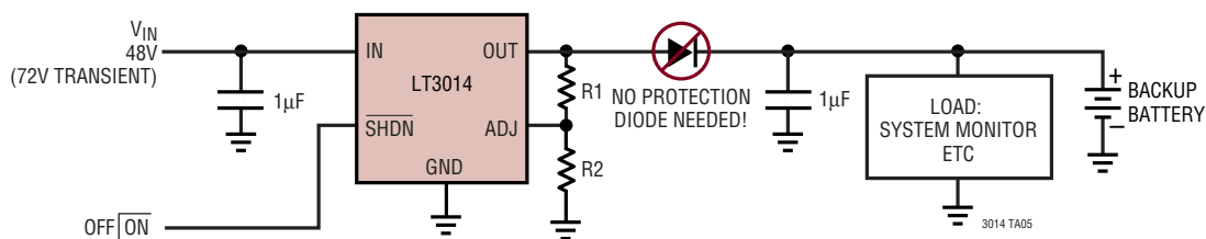
LT3014 Telecom Application
