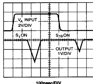
Figure 6. Break-Before-Make Delay ( t_{OPEN} )
