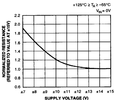
Figure 4. Normalized ON Resistance vs. Supply Voltage
