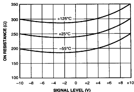
Figure 5. ON Resistance vs. Temperature
