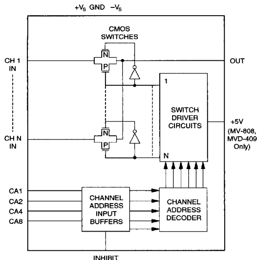
Figure 1. MV Series Functional Block Diagram
