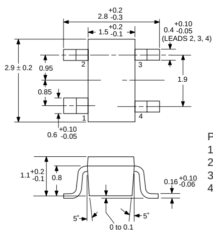
PACKAGE OUTLINE 39
