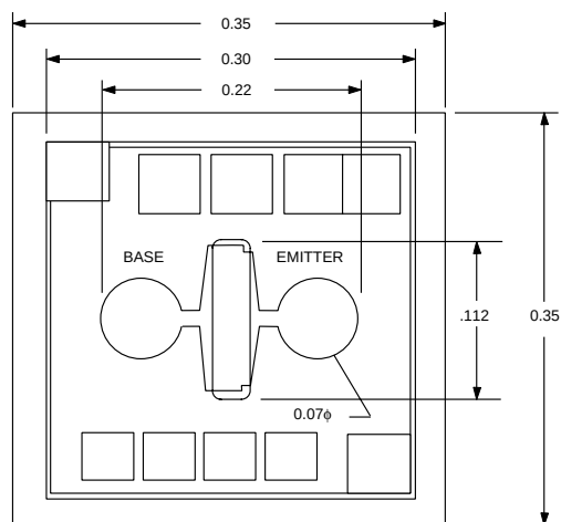
NE85600 (CHIP)
