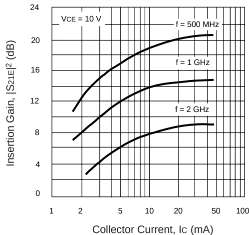
NE85635 INSERTION GAIN vs. COLLECTOR CURRENT
