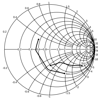
Coordinates in Ohms Frequency in GHz V_{CE} = 10\text{ V} , I_C = 10\text{ mA}
