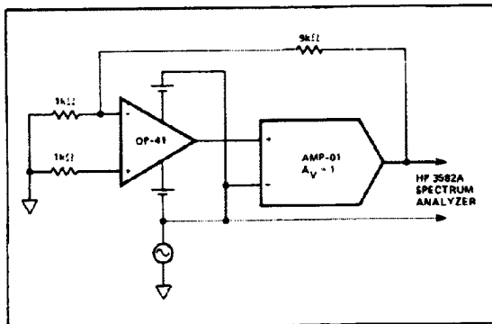
FIGURE 6: CIRCUIT USED TO MEASURE CMR FROM 10kHz TO 20kHz
