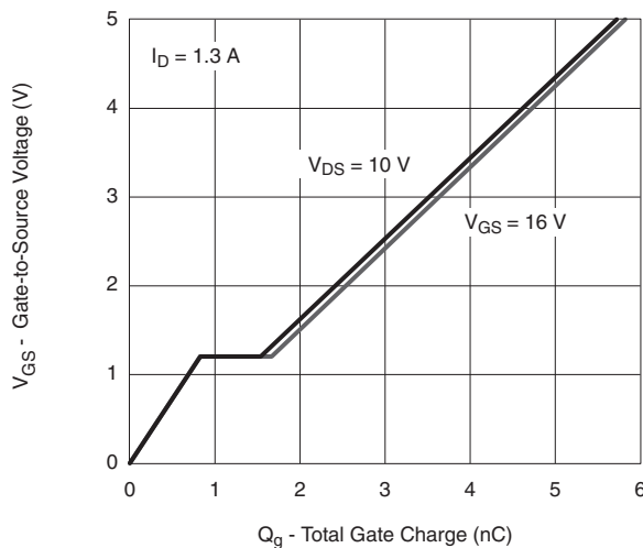
Q_g - Total Gate Charge (nC) Q_g - Gate Charge
