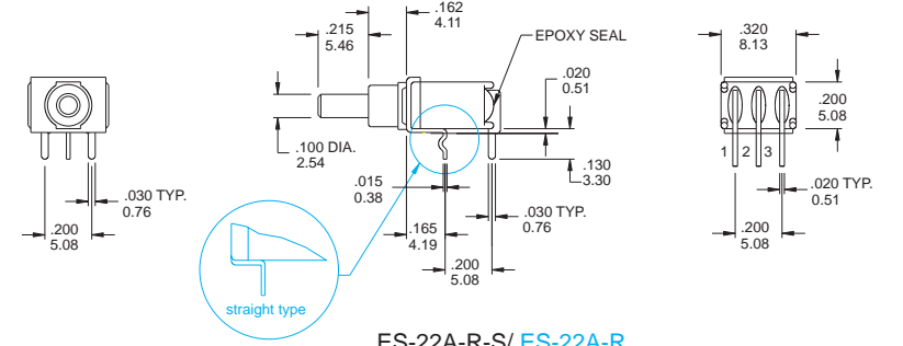
ES-22A-R-S/ ES-22A-R
