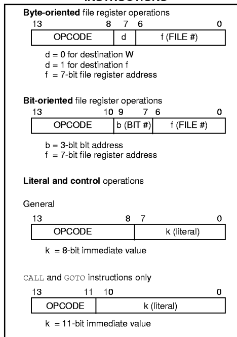
FIGURE 12-1: GENERAL FORMAT FOR INSTRUCTIONS
