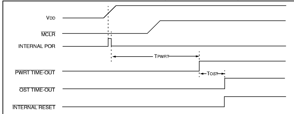
FIGURE 11-9: TIME-OUT SEQUENCE ON POWER-UP ( \overline{\text{MCLR}} NOT TIED TO \text{V}_{\text{DD}} ): CASE 2
