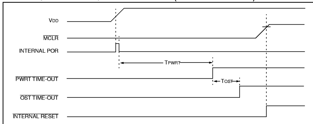
FIGURE 11-10: SLOW RISE TIME ( \overline{\text{MCLR}} TIED TO \text{V}_{\text{DD}} )
