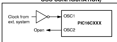
FIGURE 11-3: EXTERNAL CLOCK INPUT OPERATION (HS, XT OR LP OSC CONFIGURATION)
