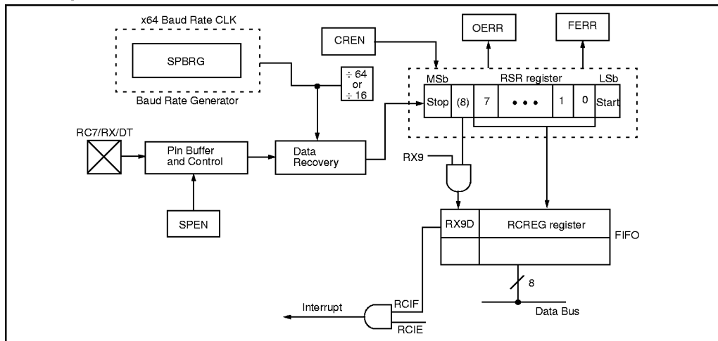
FIGURE 9-7: ASYNCHRONOUS RECEPTION
