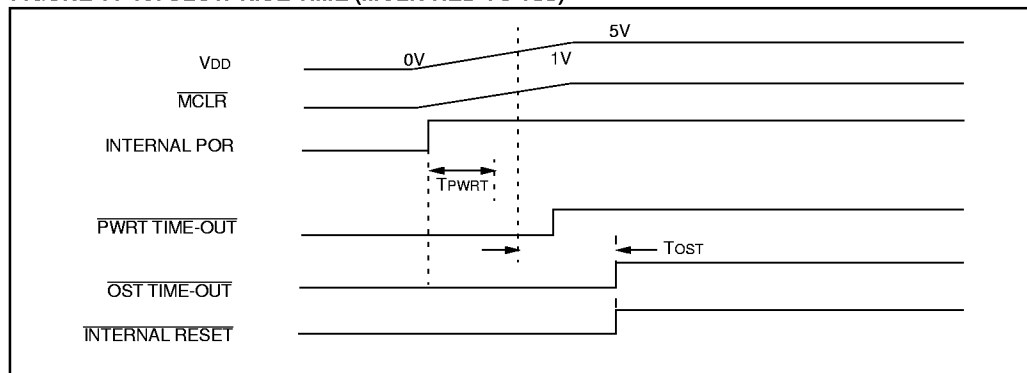
FIGURE 11-10: SLOW RISE TIME ( \overline{\text{MCLR}} TIED TO \text{V}_{\text{DD}} )
