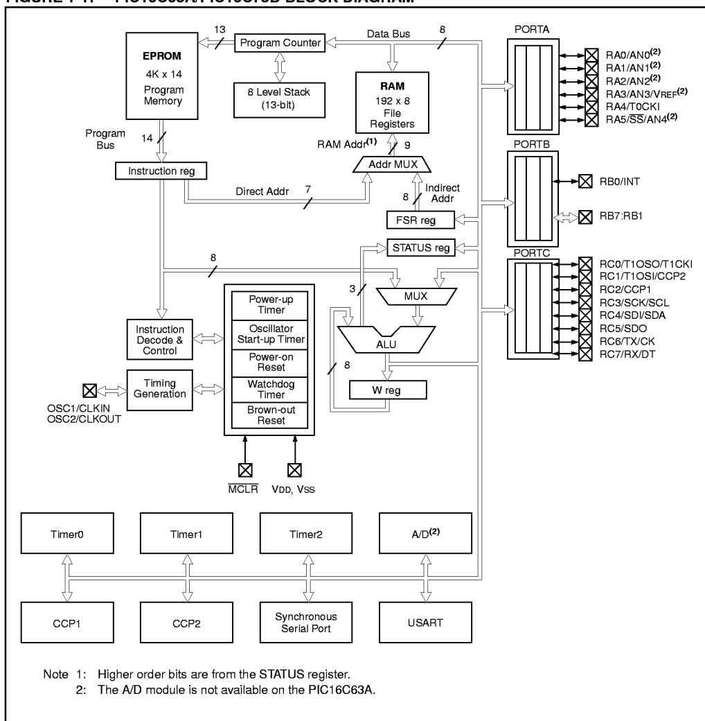
FIGURE 1-1: PIC16C63A/PIC16C73B BLOCK DIAGRAM
