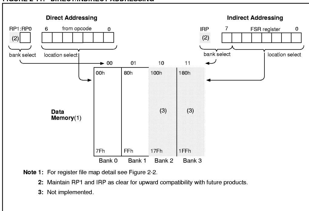
FIGURE 2-11: DIRECT/INDIRECT ADDRESSING
