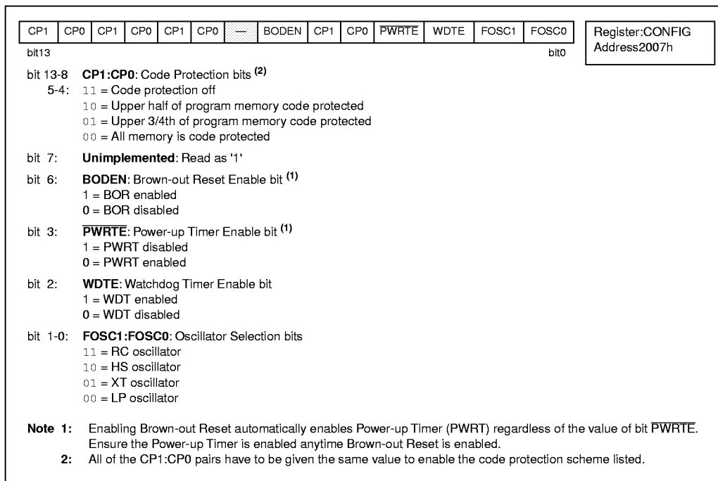
FIGURE 11-1: CONFIGURATION WORD
