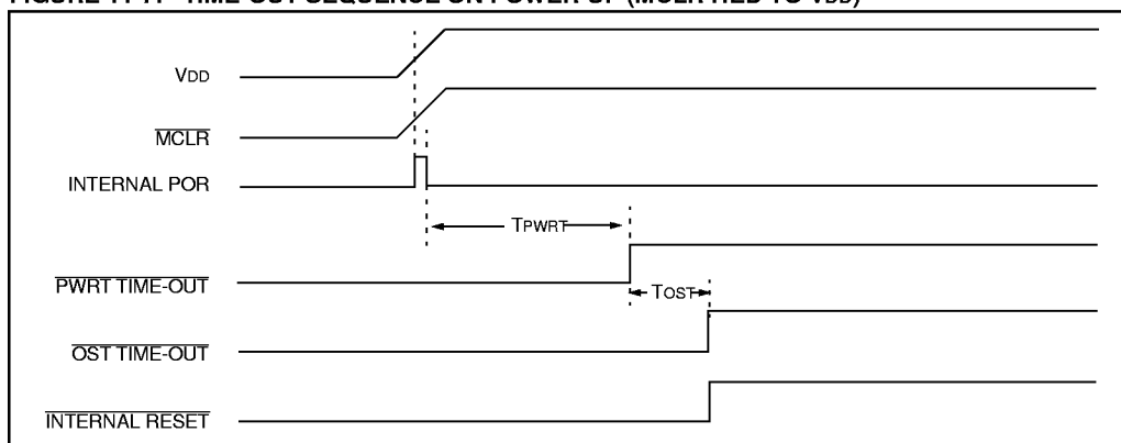
FIGURE 11-7: TIME-OUT SEQUENCE ON POWER-UP (MCLRTIED TO VDD)
