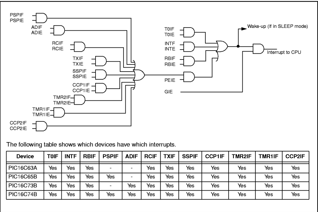
FIGURE 11-11: INTERRUPT LOGIC
