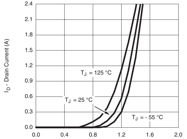
Transfer Characteristics Curves vs. Temp
