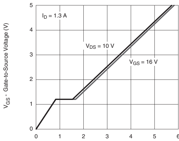
Q_g - Gate Charge
