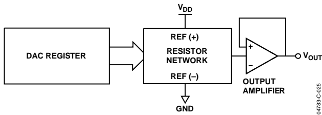
Figure 24. DAC Architecture
