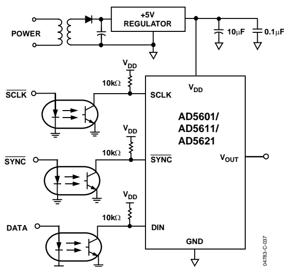
Figure 36. AD5601/AD5611/AD5621 with an Opto-Isolated Interface
