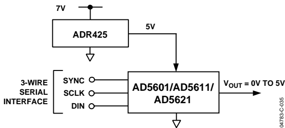
Figure 34. ADR425 as Power Supply to the AD5601/AD5611/AD5621
