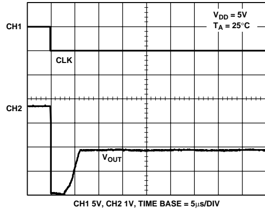
Figure 20. Exiting Power-Down
