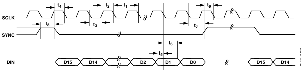
Figure 2. Timing Diagram
