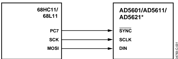
Figure 30. AD5601/AD5611/AD5621 to 68HC11/68L11 Interface
