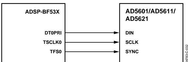
Figure 31. AD5601/AD5611/AD5621 to Blackfin ADSP-BF53X Interface
