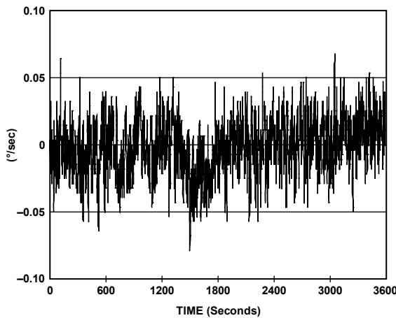
Figure 20. Typical Shift in Short Term Null (Bandwidth = 1 Hz)
