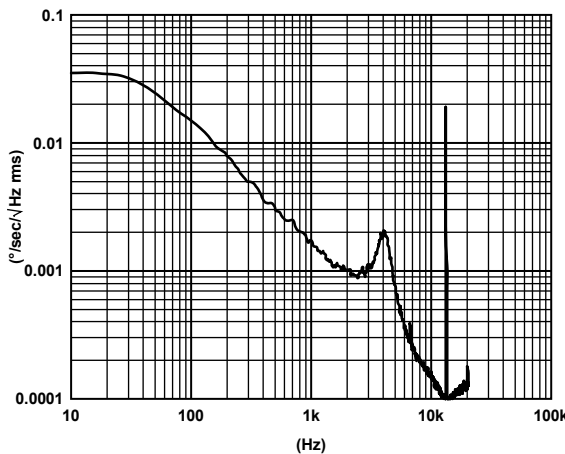
Figure 21. Typical Noise Spectral Density (Bandwidth = 40 Hz)
