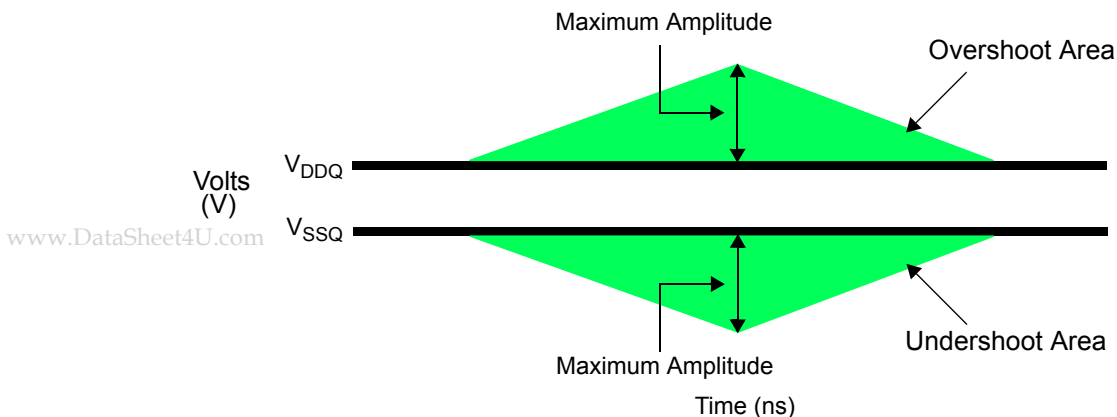
Figure 10. Clock, Data, Strobe and Mask Overshoot and Undershoot definition
