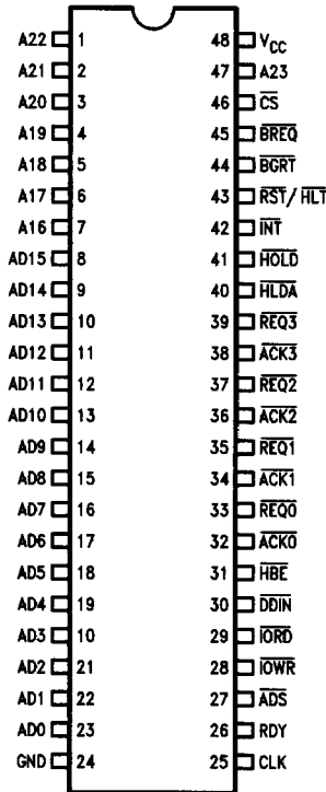
Top View
