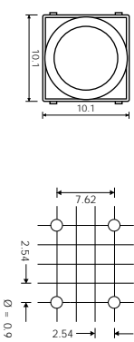
PCB layout
