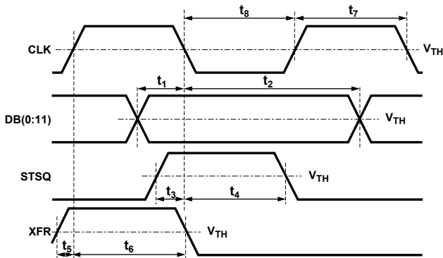
Figure 4. Timing Requirement E/O = LOW
