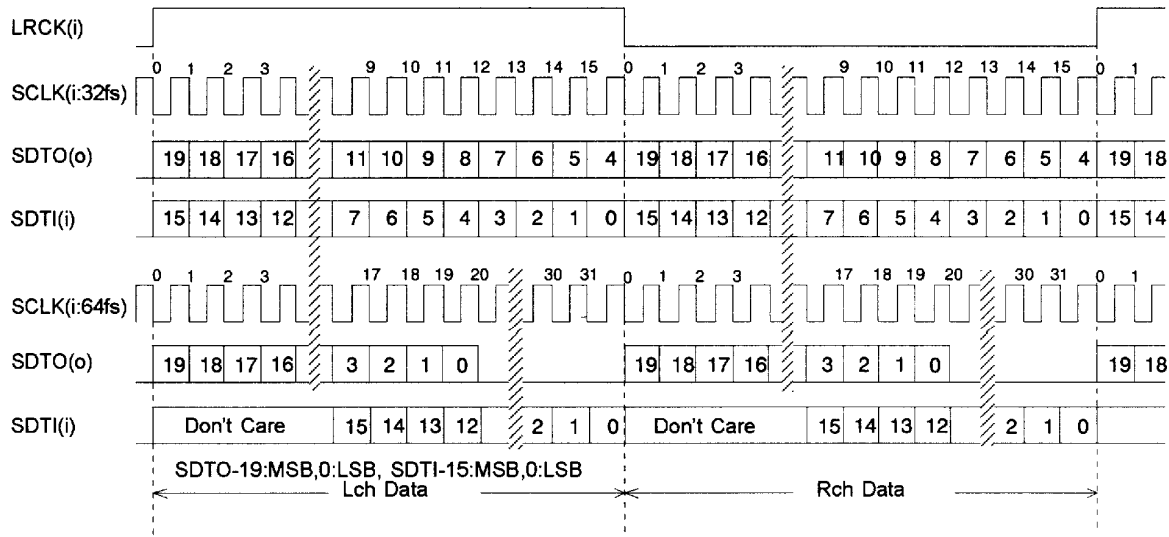
Figure 1. Mode 0 Timing
