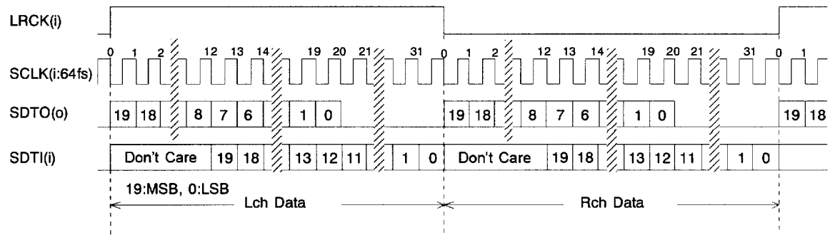
Figure 2. Mode 1 Timing
