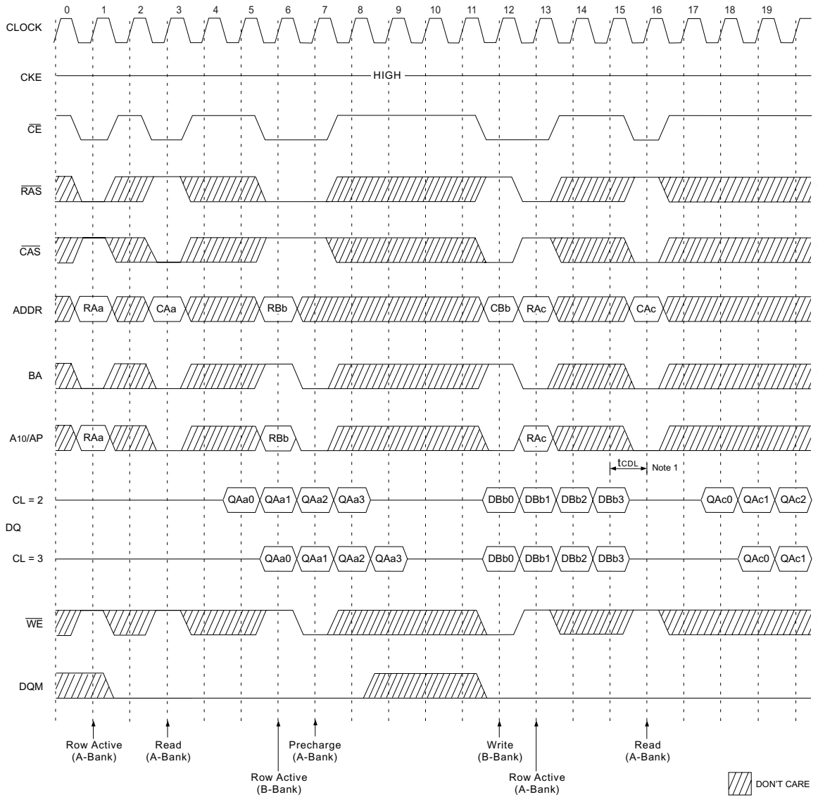
FIG. 8 READ & WRITE CYCLE AT DIFFERENT BANK @ BURST LENGTH=4
