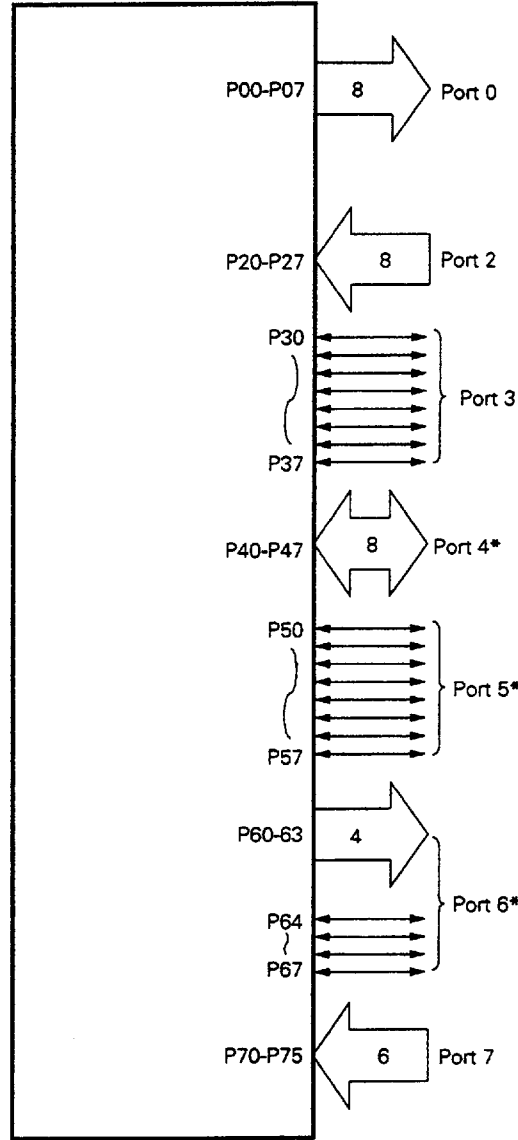
Fig. 2-3 Port Configuration
