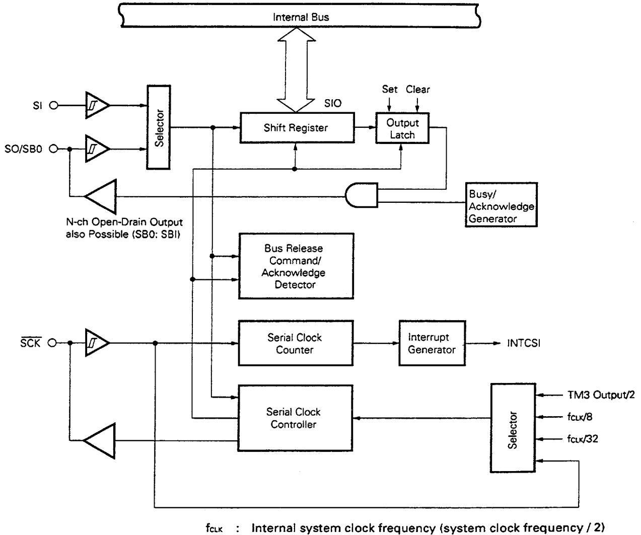
Fig. 2-9 Clocked Serial Interface Block Diagram
